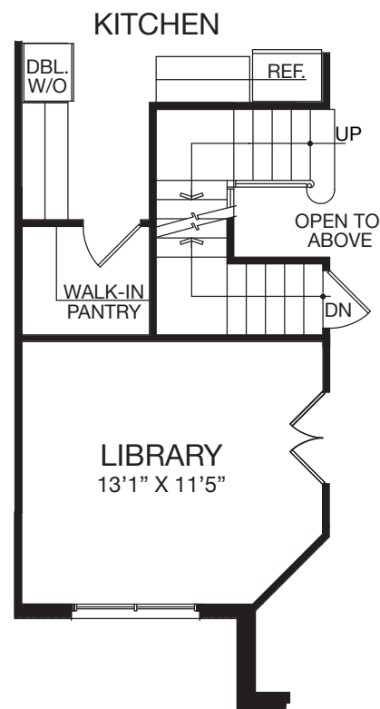
PARTIAL MAIN LEVEL W/ WALK-IN PANTRY & OPT. LIBRARY
