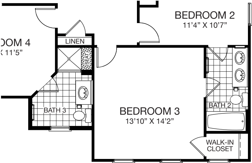
PARTIAL UPPER LEVEL W/ OPTIONAL THIRD BATH AND BUDDY BATH
