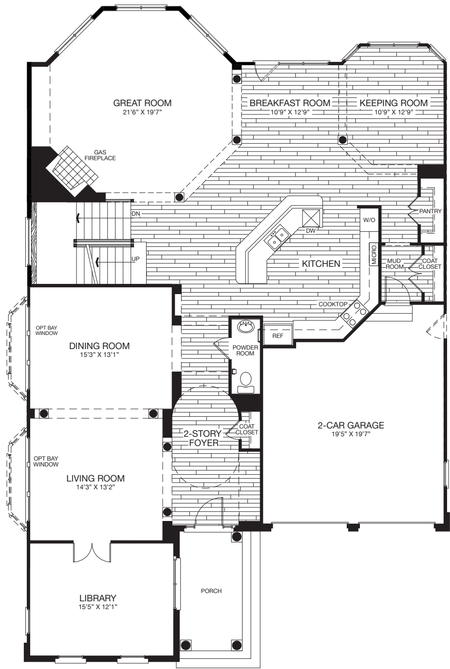
THE BUXTON FIRST FLOOR PLAN
