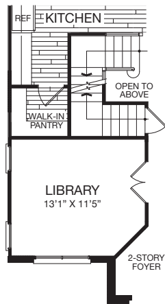
PARTIAL MAIN LEVEL W/ OPT. LIBRARY & WALK-IN PANTRY
